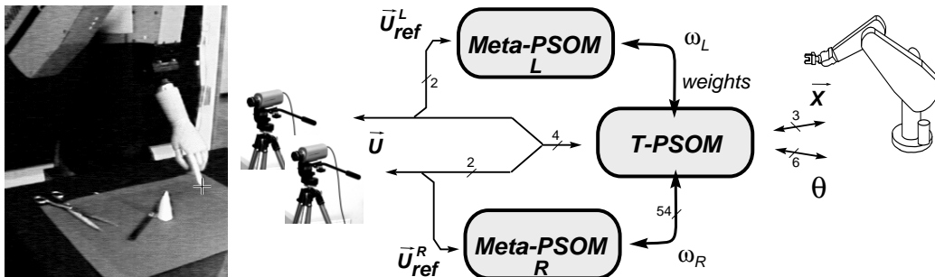
Figure 9.7: Rapid learning of the 3D visuo-motor coordination for two cameras. The basis T-PSOM ( m = 3 ) is capable of mapping to and from three coordinate systems: Cartesian robot world coordinates, the robot joint angles (6-DOF), and the location of the end-effector in coordinates of the two camera retinas. Since the left and right camera can be relocated independently, the weight set of T-PSOM is split, and parts \omega_L, \omega_R are learned in two separate Meta-PSOMs (“L” and “R”).
