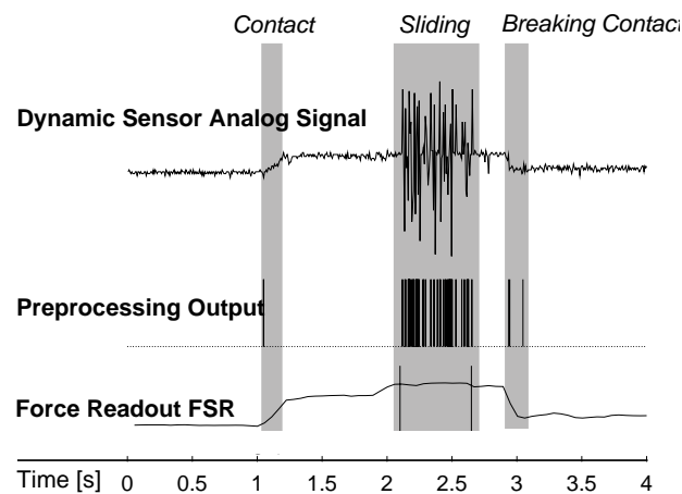
Figure 2.9: Recordings from the raw and pre-processed signal of the dynamic slippage sensor. A flat wooden object is pressed against the sensor, and after a short rest tangentially drawn away. By band-pass filtering the slip signal of interest can be extracted: The middle trace clearly shows the sudden contact and the slippage phase. The lower trace shows the force values obtained from the second sensor.
