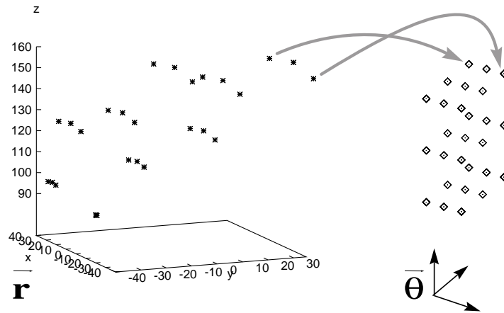
Figure 8.4: The 27 training data vectors for the Back-propagation networks: (left) in the input space \vec{r} and (right) the corresponding target output values \vec{\theta} .
