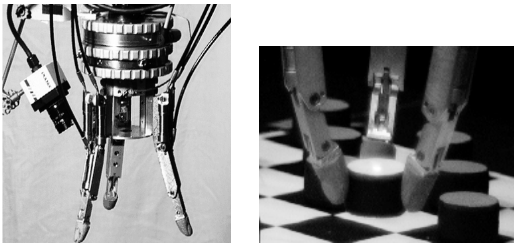
Figure 2.4: The endeffector. ( left: ) Between the arm and the hydraulic hand, the cylinder shaped FTS device can measure current 6D force torque values. The three finger modules are mounted here symmetrically at the 12 sided regular prism base. On the left side, the color video camera looks at the scene from an end-effector fixed position. Inside the flat palm, a diode laser is directed in tool axis, which allows depth triangulation in the viewing angle of the camera.
