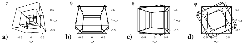
Figure 7.2: The \phi, \theta, \psi, z system. (a) The cubical test object seen by the camera when rotated and shifted in several depths z ( \phi=10^\circ, \theta=20^\circ, \psi=30^\circ, z=2 \dots 6L , cube size L .) (b–d) 0^\circ, 20^\circ , and 30^\circ rotations in the roll \phi , pitch \theta , and yaw \psi system. (The transformations are applied from right to left \psi, \theta, \phi, z .)
